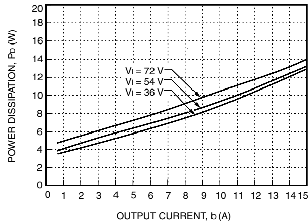
Figure 30. JFW075A Power Dissipation vs. Output Current at 25 °C
