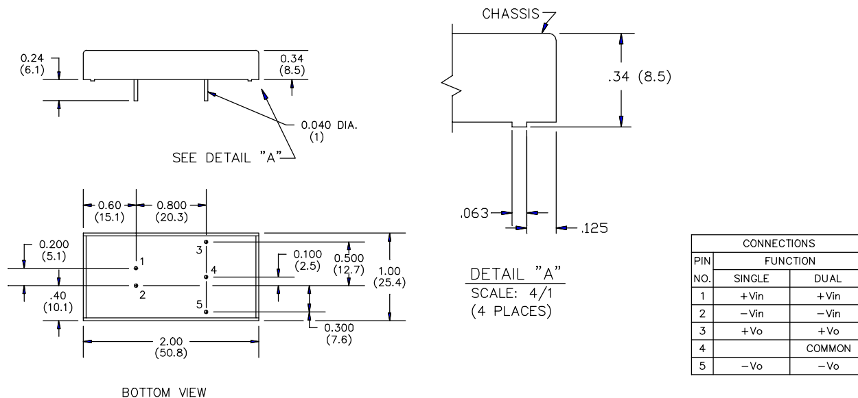
BOTTOM VIEW
