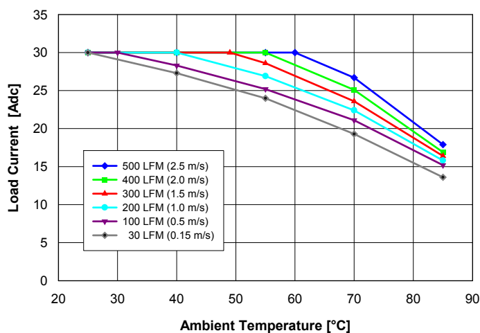
Fig. 12: Available load current vs. ambient temperature and airflow rates for converter mounted horizontally with V_{in} = 54 V, air flowing from pin 3 to pin 4 and maximum FET temperature \leq 105^{\circ}\text{C} .
