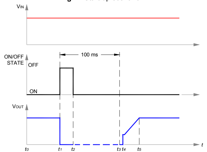
Fig. 8: Start-up scenario #3.
