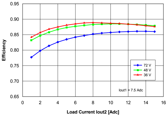
Fig. 14: Efficiency vs. load current lout2 and input voltage for converter mounted vertically with air flowing from pin 3 to pin 1 at a rate of 300 LFM (1.5 m/s), for lout1 = 7.5 A and Ta = 25°C.
