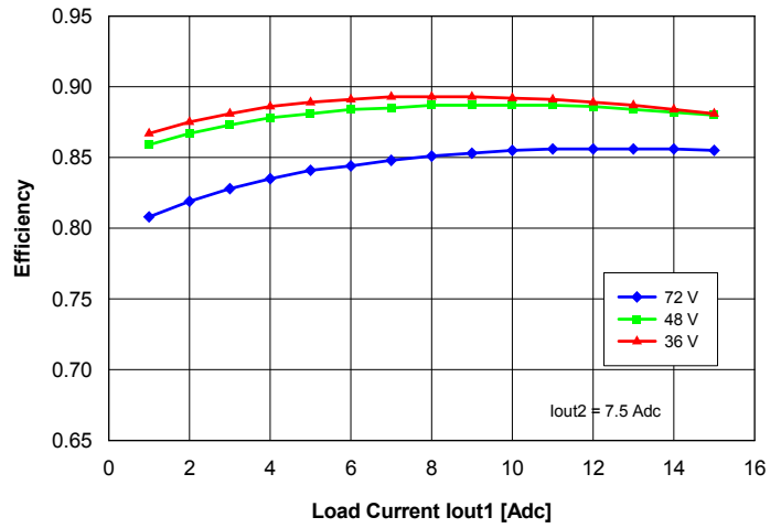
Fig. 13: Efficiency vs. load current lout1 and input voltage for converter mounted horizontally with air flowing from pin 3 to pin 4 at a rate of 300 LFM (1.5 m/s), for lout2 = 7.5 A and Ta = 25°C.
