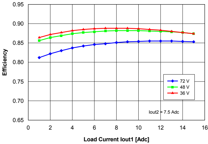
Fig. 12: Efficiency vs. load current lout1 and input voltage for converter mounted vertically with air flowing from pin 3 to pin 1 at a rate of 300 LFM (1.5 m/s), for lout2 = 7.5 A and Ta = 25°C.
