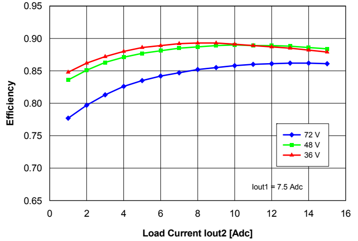
Fig. 15: Efficiency vs. load current lout2 and input voltage for converter mounted horizontally with air flowing from pin 3 to pin 4 at a rate of 300 LFM (1.5 m/s), for lout1 = 7.5 A and Ta = 25°C.
