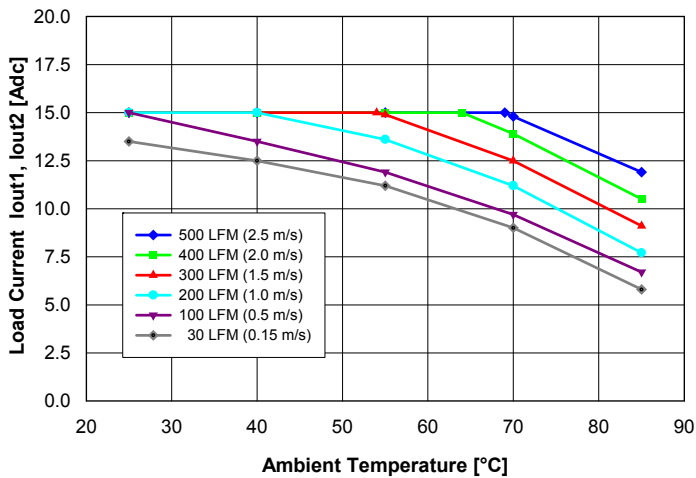
Fig. 10: Available balanced load current (Iout1 = Iout2) vs. ambient air temperature and airflow rates for converter mounted vertically with Vin = 48 V, air flowing from pin 3 to pin 1 and maximum FET temperature ≤ 120°C.
