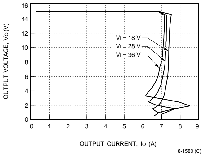
Figure 4. Typical JC100C Output Characteristics at Room Temperature
