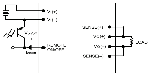
Figure 16. Remote On/Off Implementation
