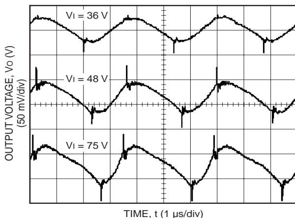
Figure 21. Output Ripple Voltage ( I_O = I_{O, \text{max}} ).
