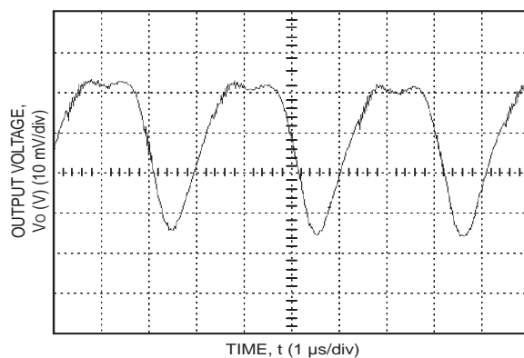
Figure 33. Output Ripple Voltage ( I_O = I_{O, \text{max}} ).
