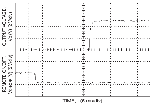
Figure 36. Start-up from Remote On/Off ( I_O = I_{O, \text{max}} ).
