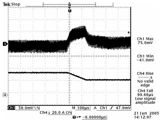
Vout=1.5 V, 75% to 50% Load Transients
