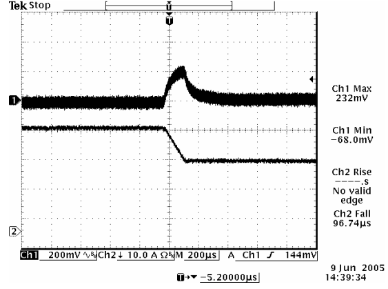
Vout=5 V, 75% to 50% Load Transients
