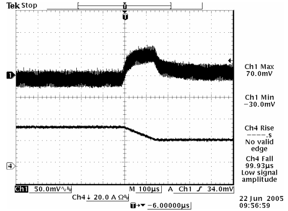
Vout=1.2 V, 75% to 50% Load Transients
