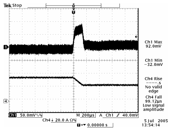
Vout=2.5 V, 75% to 50% Load Transients
