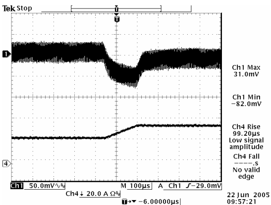
Vout=1.5 V, 50% to 75% Load Transients
