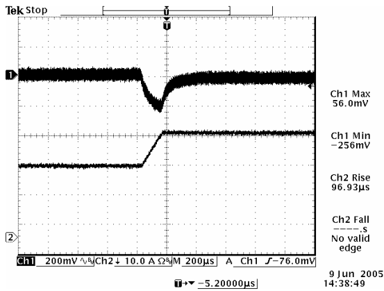
Vout=5 V, 50% to 75% Load Transients
