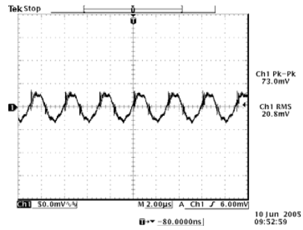
48 Vdc input, 5 Vdc/48 A output
