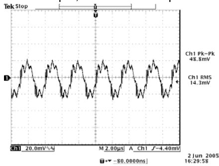
48 Vdc input, 3.3 Vdc/70 A output
