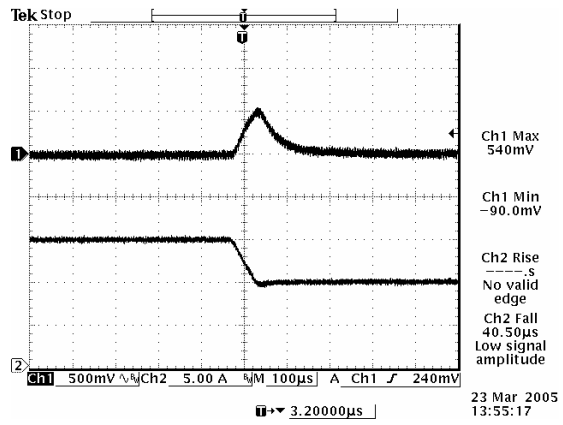
Vout=12 V, 75% to 50% Load Transients
