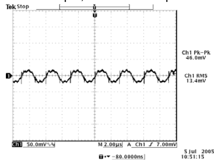
48 Vdc input, 2.5 Vdc/80 A output
