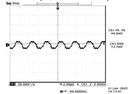
48 Vdc input, 1.5 Vdc/80 A output
