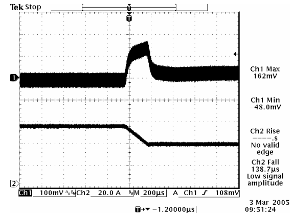
Vout=3.3 V, 75% to 50% Load Transients
