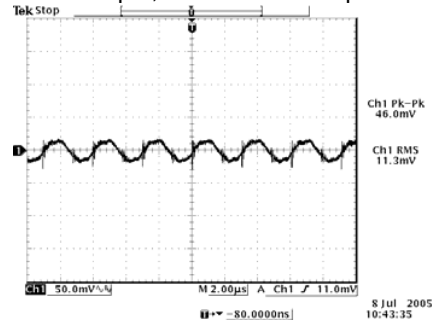
48 Vdc input, 1.8 Vdc/80 A output
