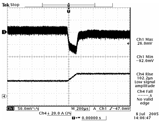
Vout=1.8 V, 50% to 75% Load Transients
