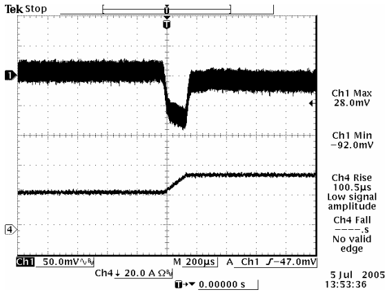
Vout=2.5 V, 50% to 75% Load Transients
