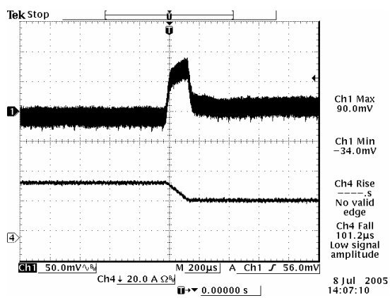
Vout=1.8 V, 75% to 50% Load Transients
