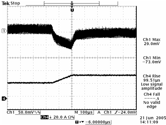
Vout=1.2 V, 50% to 75% Load Transients
