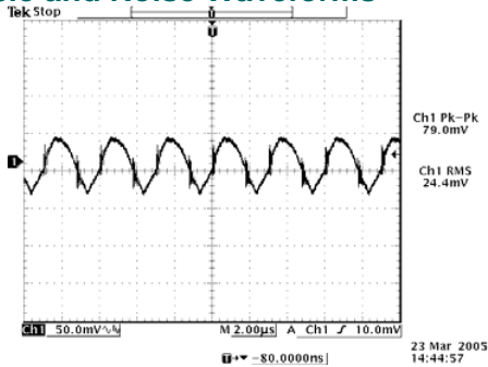
48 Vdc input, 12 Vdc/20 A output
