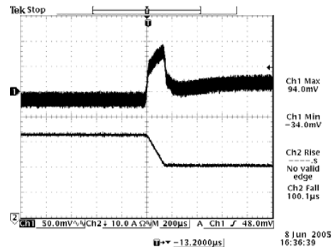
Vout= 1.8 V 75%-50% Load Transients
