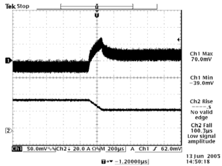
Vout= 1.2 V 75%-50% Load Transients
