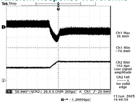
Vout= 1.2 V 50%-75% Load Transients
