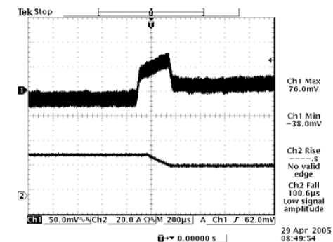
Vout= 2.5 V 75%-50% Load Transients
