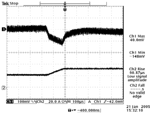
Vout= 3.3 V 50%-75% Load Transients
