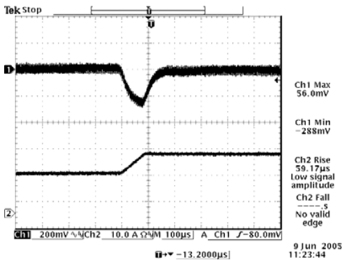
Vout= 5.0 V 50%-75% Load Transients
