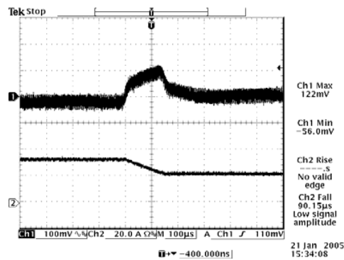
Vout= 3.3 V 75%-50% Load Transients
