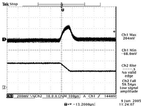
Vout= 5.0 V 75%-50% Load Transients
