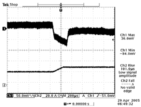
Vout= 2.5 V 50%-75% Load Transients
