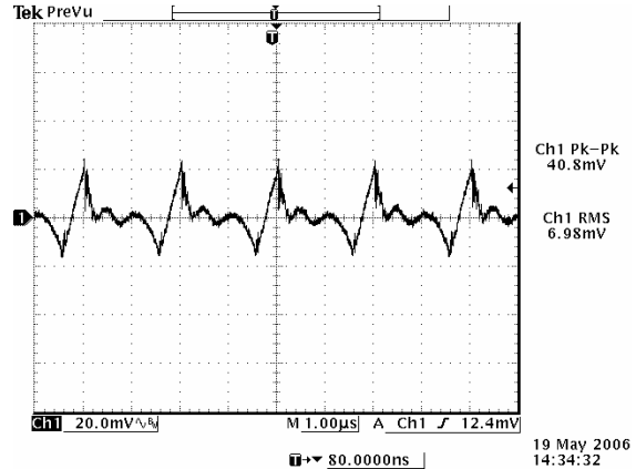
48 Vdc input, 3.3 Vdc output
