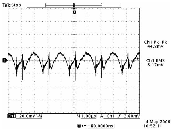
48 Vdc input, 5.0 Vdc output
