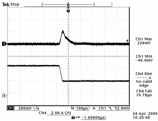
Vout=3.3 V 50% to 25% Load Transients
