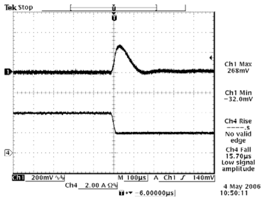
Vout=5.0 V 50% to 25% Load Transients
