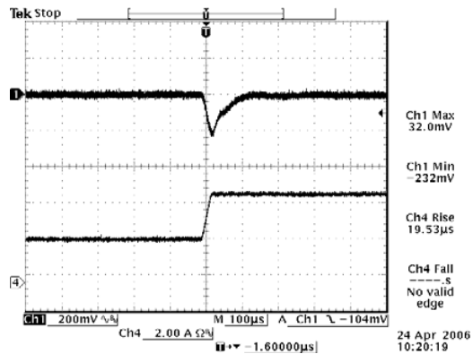
Vout=3.3 V 25% to 50% Load Transients
