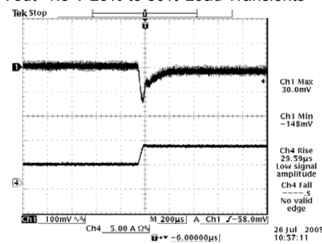
Vout=3.3 V 50% to 25% Load Transients
