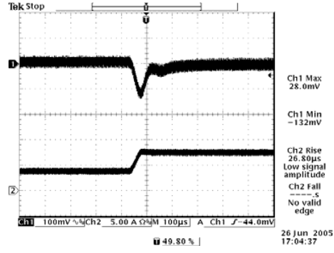
Vout=1.8 V 25% to 50% Load Transients
