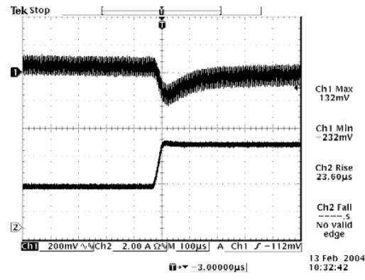
Vout=5.0 V 25% to 50% Load Transients
