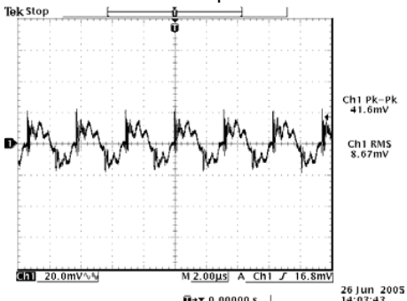
1.8 V/15 A output.
