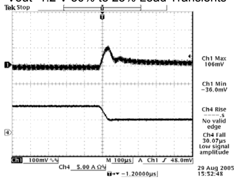
Vout=1.2 V 25% to 50% Load Transients
