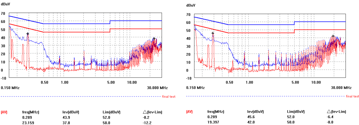
Figure 23. EMC Filter
