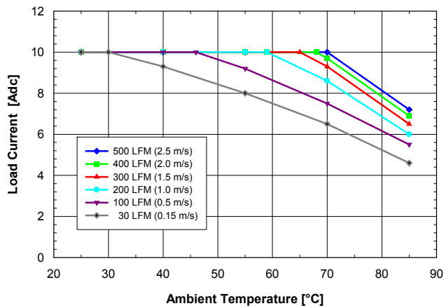
Fig. 5.0V.2: Available load current vs. ambient air temperature and airflow rates for SQ48T10050 converter with D height pins mounted horizontally with V_{in} = 48\text{ V} , air flowing from pin 3 to pin 1, and maximum FET temperature \leq 120^\circ\text{C} .
