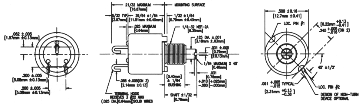
Figure 9 Series 392M/RV6 Dimensions
