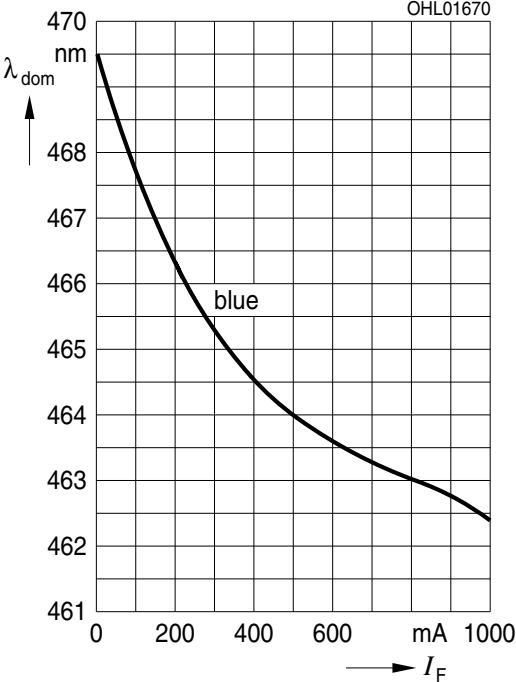
Dominant Wavelength 2) page 16
