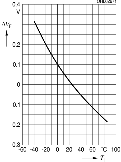
Relative Forward Voltage 2) page 16
