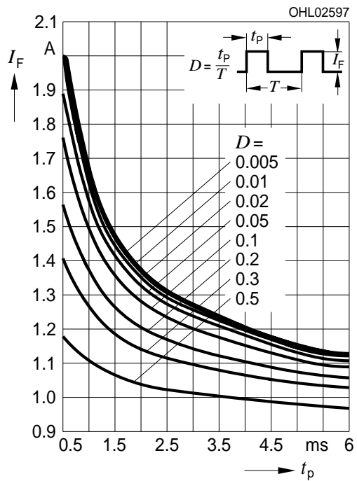
Zulässige Impulsbelastbarkeit I_F = f(t_p) Permissible Pulse Handling Capability blue Duty cycle D = parameter, T_{board} = 85\text{ °C} 1 chip operated
