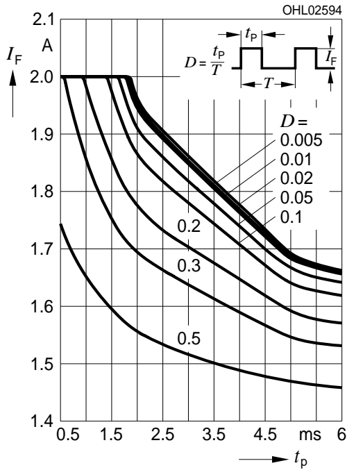
Zulässige Impulsbelastbarkeit I_F = f(t_p) Permissible Pulse Handling Capability amber Duty cycle D = parameter, T_{board} = 85\text{ °C} 1 chip operated
