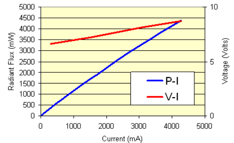
LIV Graph
