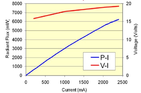
LIV Graph
