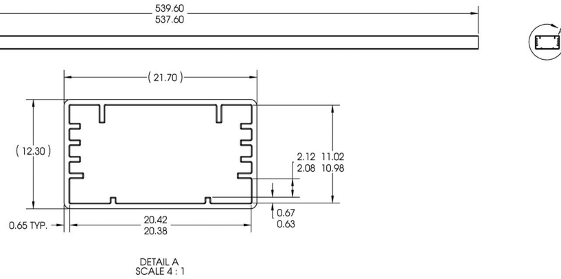
Figure 38: Tube Design for Hexagonal Star Products
