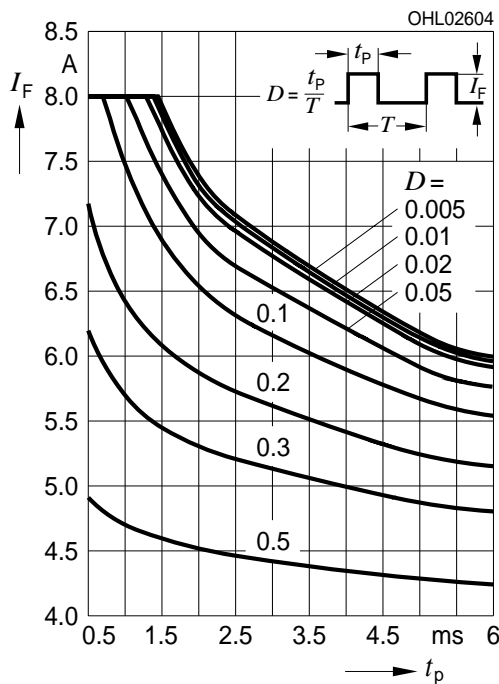
Zulässige Impulsbelastbarkeit I_F = f(t_p) Permissible Pulse Handling Capability blue, true green Duty cycle D = parameter, T_{board} = 25^\circ\text{C} 4 chips operated parallel; current for single chip is I_f/4
