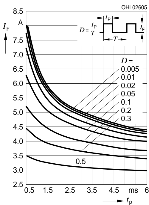
Zulässige Impulsbelastbarkeit I_F = f(t_p) Permissible Pulse Handling Capability blue, true green Duty cycle D = parameter, T_{board} = 85^\circ\text{C} 4 chips operated parallel; current for single chip is I_f/4
