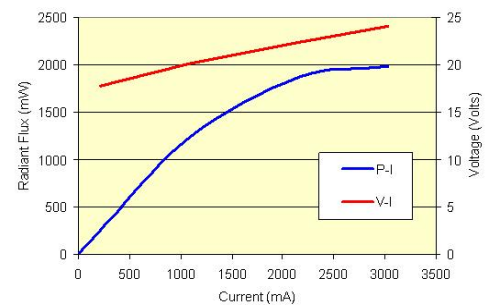
LIV Graph
