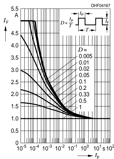
Zulässige Impulsbelastbarkeit Permissible Pulse Handling Capability I_F = f(t_p), T_B = 85\text{ °C}, Duty cycle D = \text{parameter}
