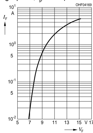
Durchlassstrom Forward Current I_F = f(V_F), T_B = 25\text{ °C}, Single pulse, t_p = 100\ \mu\text{s}
