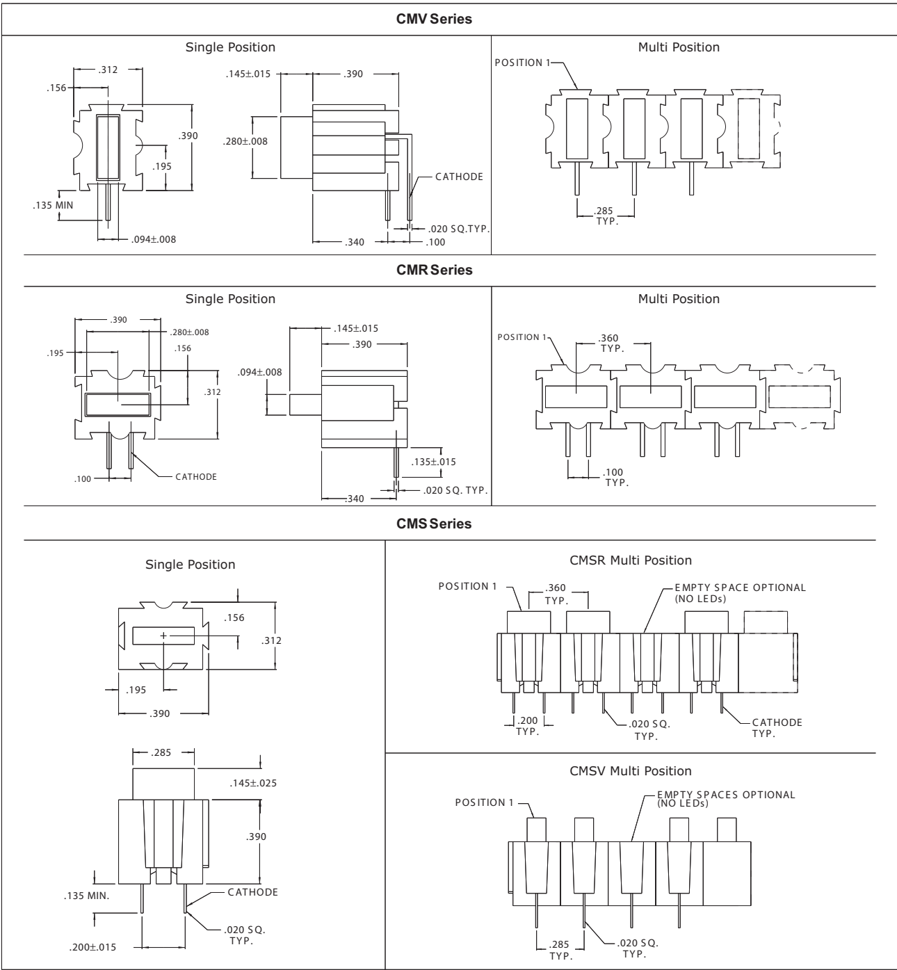
All dimensions in inches. - Mounting hole patterns on page 1-X3.
