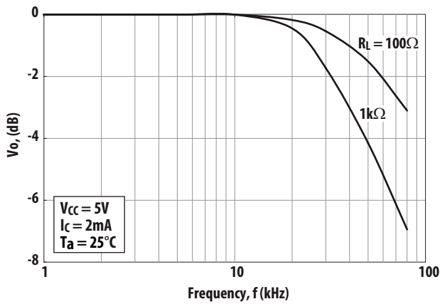
Figure 19. Frequency Response
