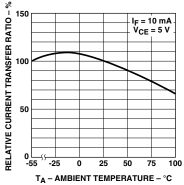
Figure 7. Relative current transfer ratio vs. temperature.
