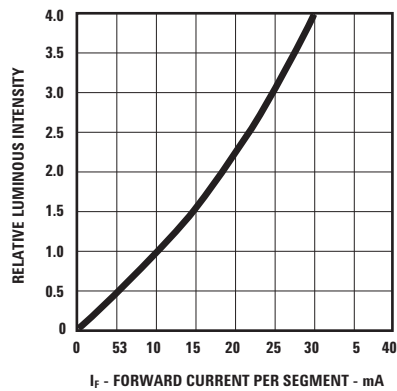
Figure 12. Relative Luminous Intensity vs. DC Forward Current.
