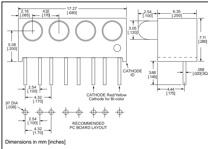
Standard Polarity shown in drawing: Cathode right
