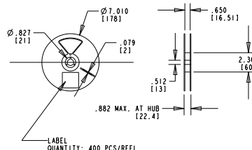
7 INCH DIA. REEL SPECIFICATIONS
