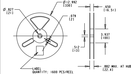
13 INCH DIA. REEL SPECIFICATIONS
