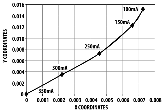
Figure 13. Chromaticity Shift vs. Current
