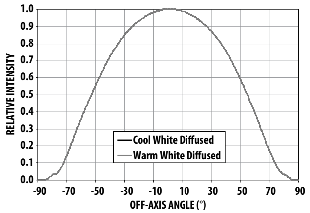
Figure 4. Radiation Pattern
