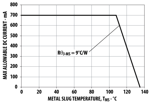
Figure 12. Maximum Forward Current vs. Metal Slug Temperature. Derated based on T JMAX = 135°C, R θJ-MS = 9°C/W
