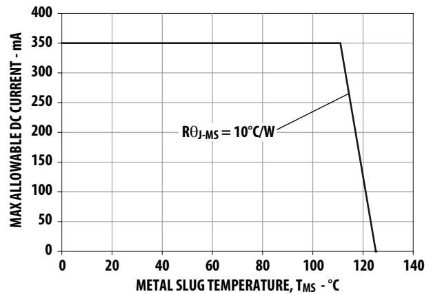
Figure 12. Maximum Forward Current vs. Metal Slug Temperature. Derated based on T_{JMAX} = 125^{\circ}\text{C} , R\theta_{JMS} = 10^{\circ}\text{C/W} .
