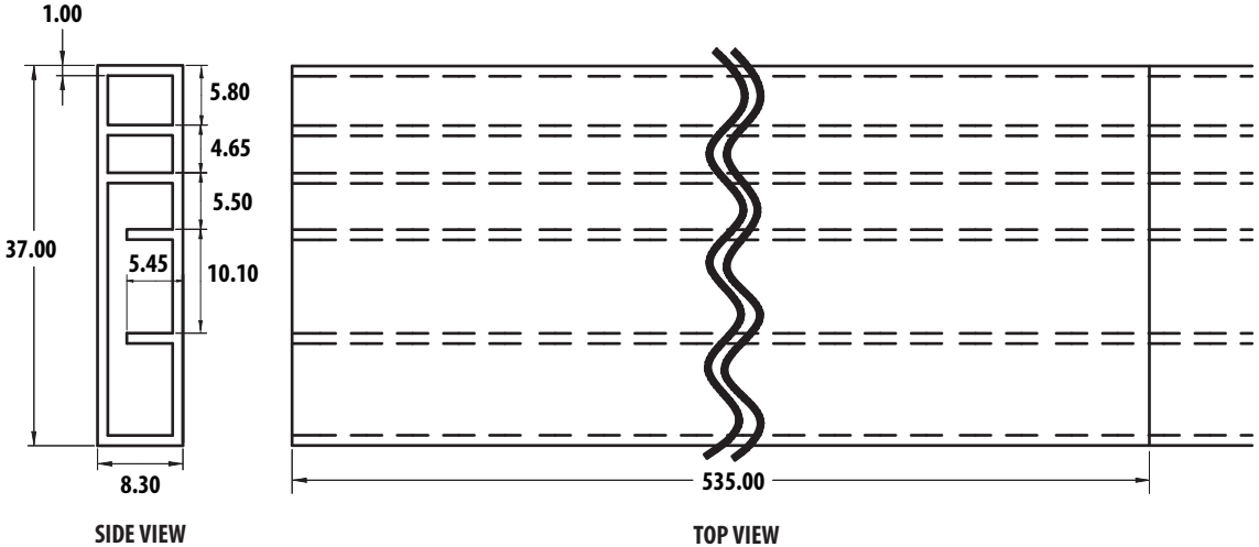
Figure 17. Tube dimensions.
