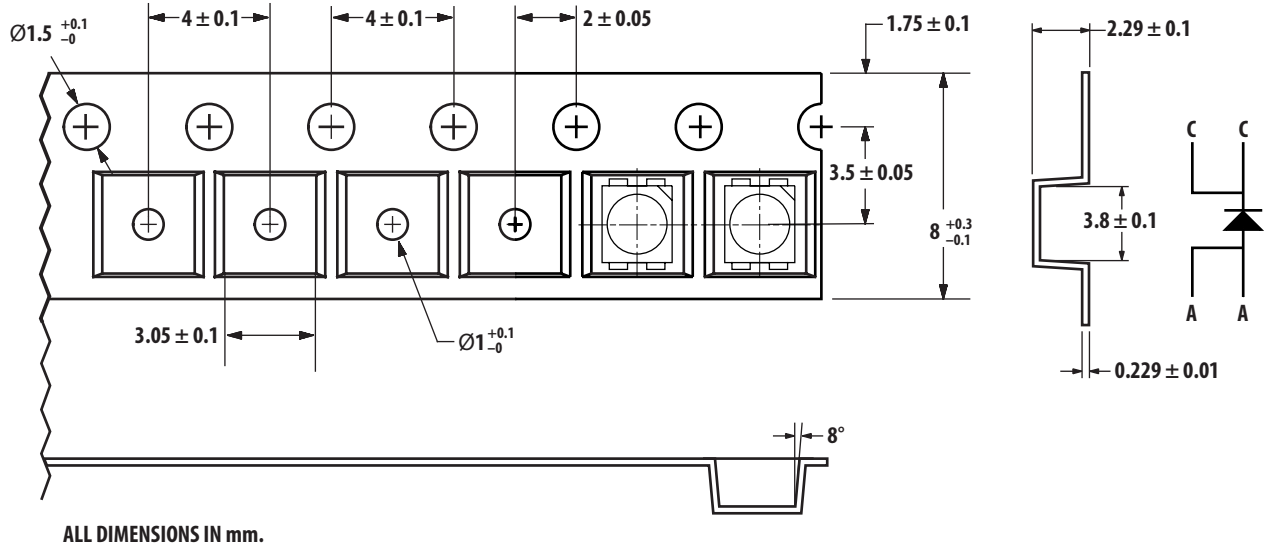
Figure 15. Tape Dimensions
