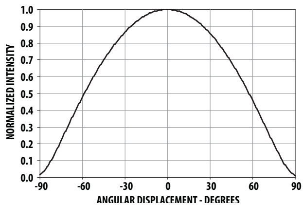
Figure 11. Radiation Pattern
