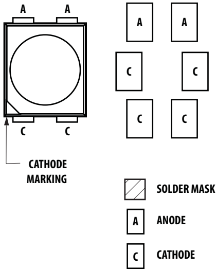
Figure 14. Recommended Soldering Pad Pattern
