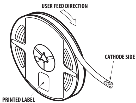
Figure 16. Reeling Orientation
