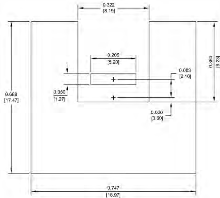
Copper Pattern
