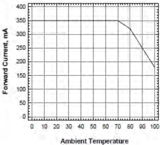
Forward Current Vs Ambient Temperature (Rja=40K/W)
