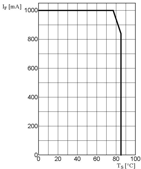
Maximal zulässiger Durchlassstrom Max. Permissible Forward Current I_F = f(T_S) ; for blue chip operated
