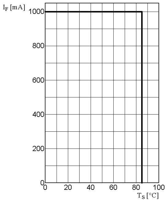
Maximal zulässiger Durchlassstrom Max. Permissible Forward Current I_F = f(T) ; for true green / blue 1 chip operated
