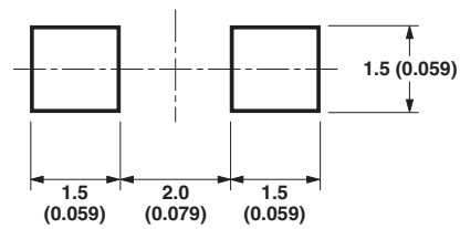
Figure 12. Recommended soldering pattern for HSMx-C152.
