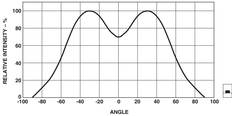
Figure 6. Relative intensity vs. angle for HSMx-C112.
