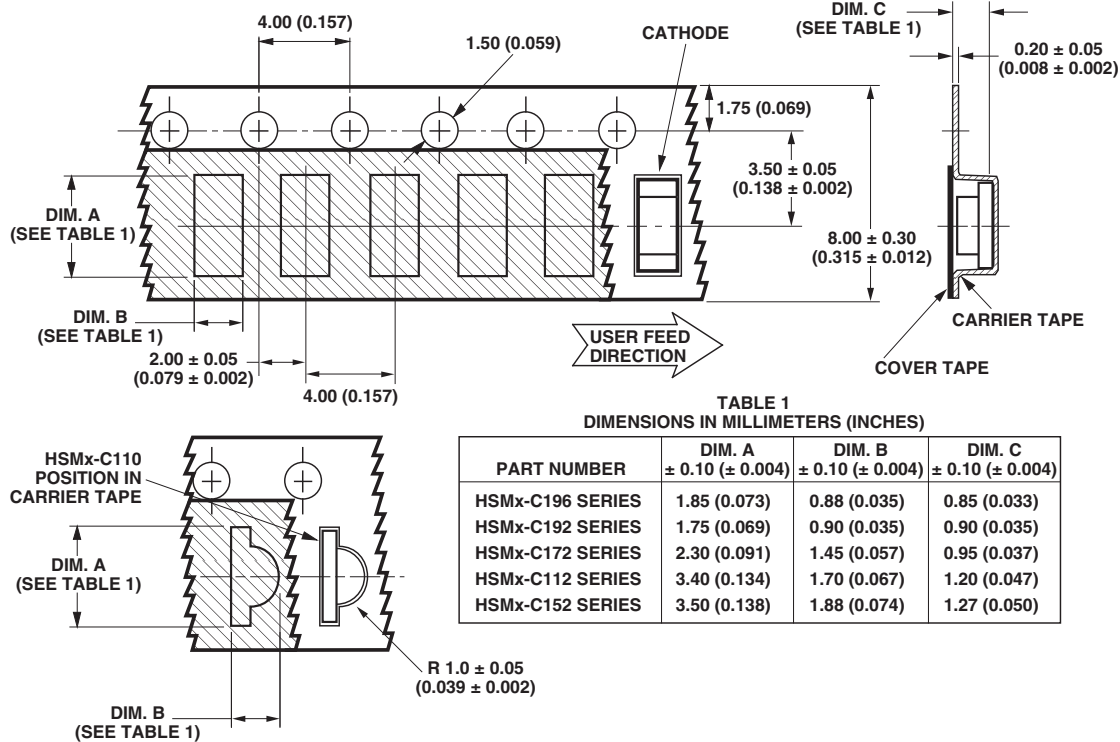
Figure 15. Tape dimensions.
