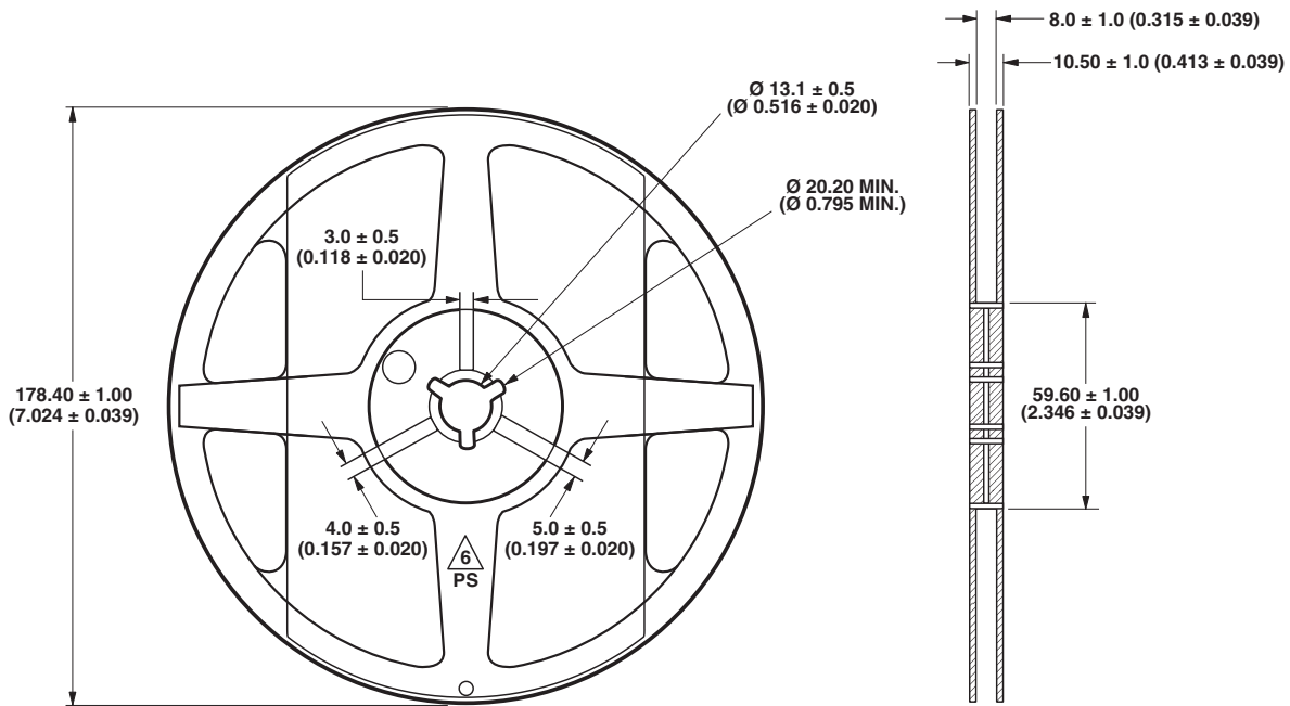
Figure 14. Reel dimensions.
