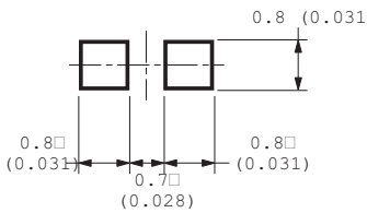
Figure 10. Recommended Soldering Pattern for HSMB-C190 and C191.
