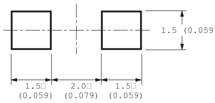
Figure 12. Recommended Soldering Pattern for HSMB-C150.
