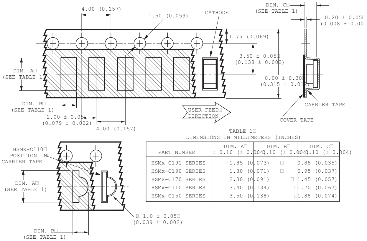
Figure 15. Tape Dimensions.
