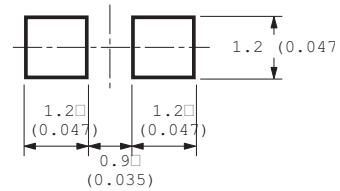
Figure 9. Recommended Soldering Pattern for HSMB-C170.
