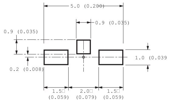
Figure 11. Recommended Soldering Pattern for HSMB-C110.
