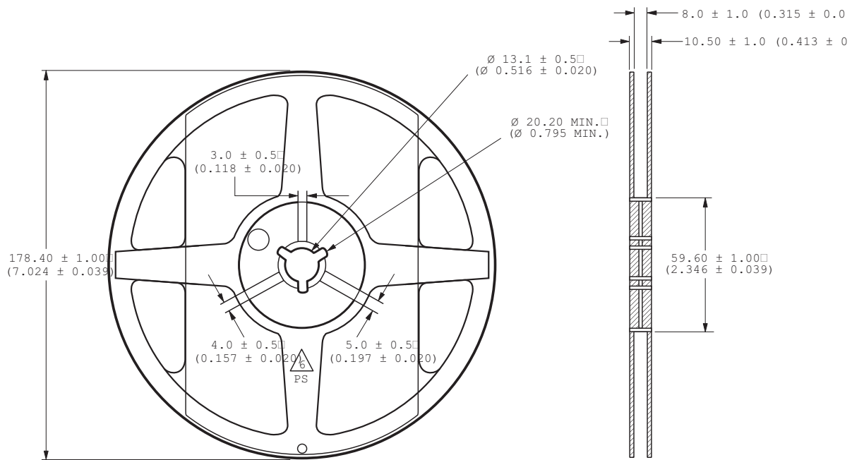
Figure 14. Reel Dimensions.
