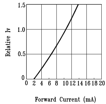
Fig.3 Relative Luminous Intensity vs. Applied Forward Voltage 12 Volts Devices
