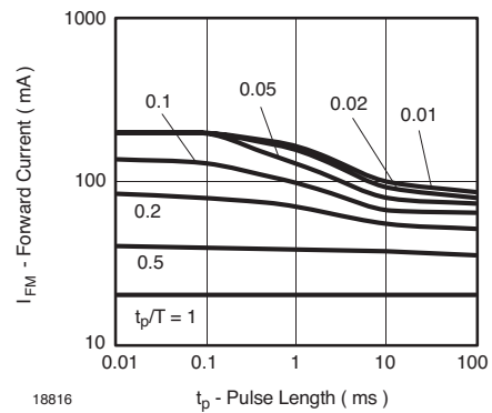
Figure 8. Forward Current vs. Pulse Length
