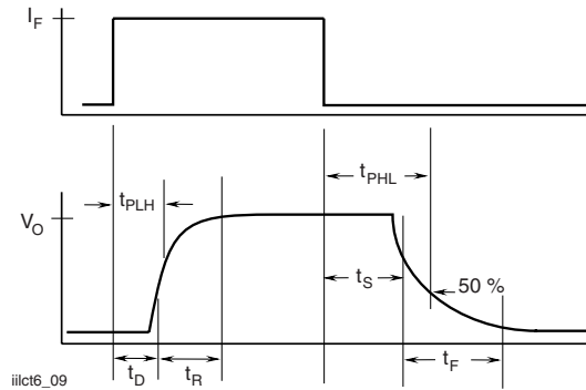
Fig. 9 - Switching Timing
