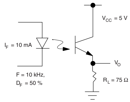
Fig. 10 - Switching Schematic
