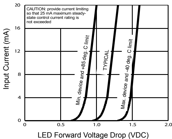
Figure 5. Input Characteristics
