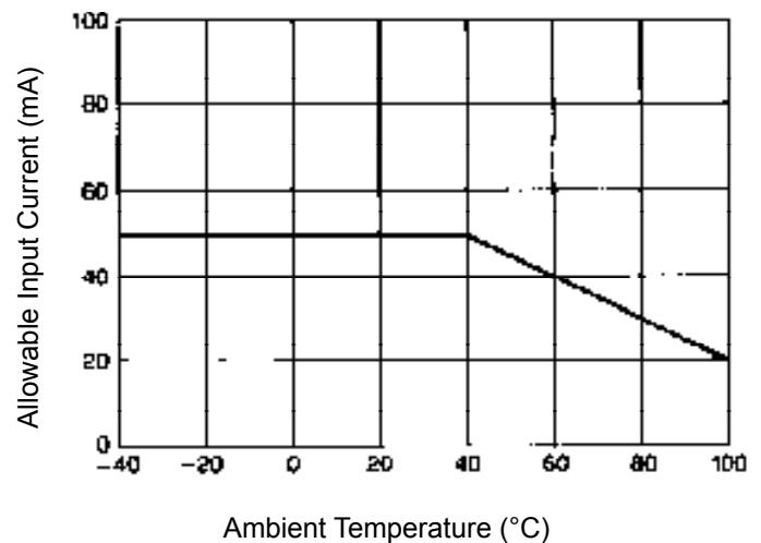
Figure 4. Input Current Derating
