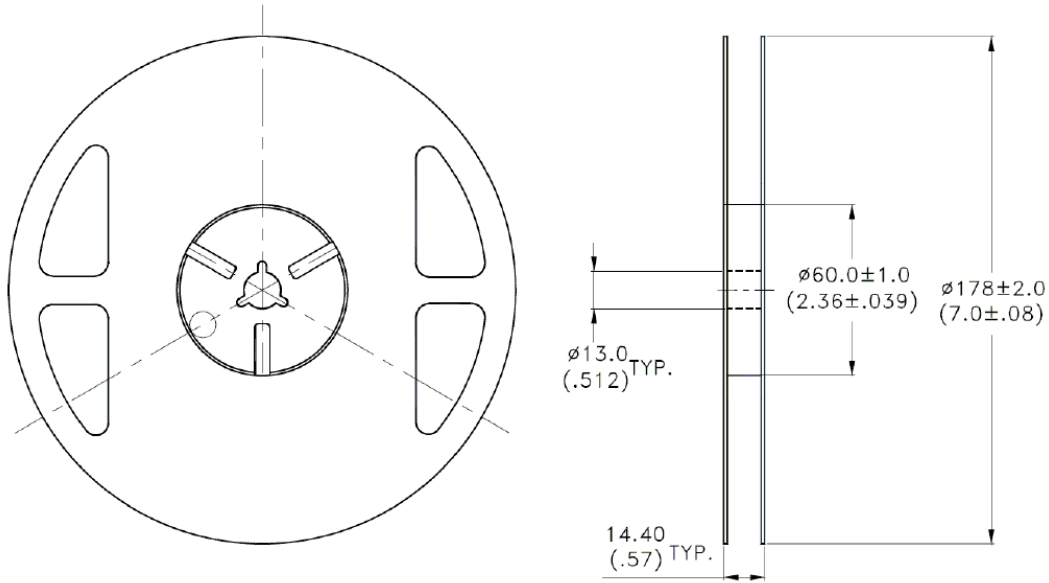
Figure 9. Reel Dimensions
