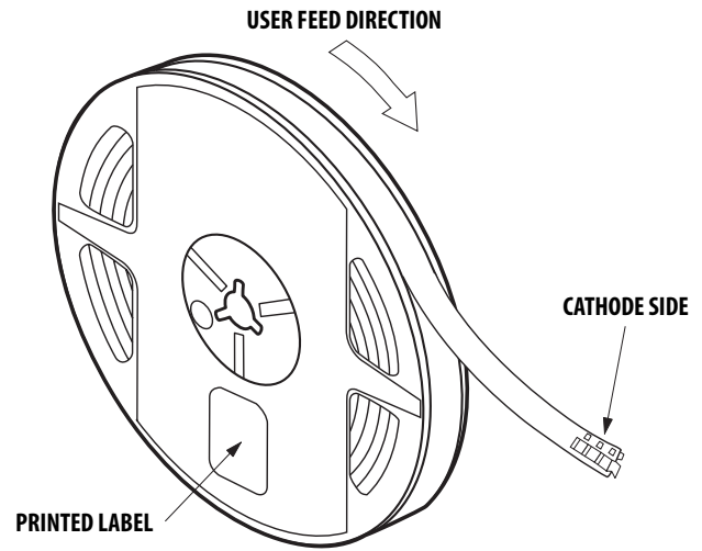
Figure 8. Reeling Orientations
