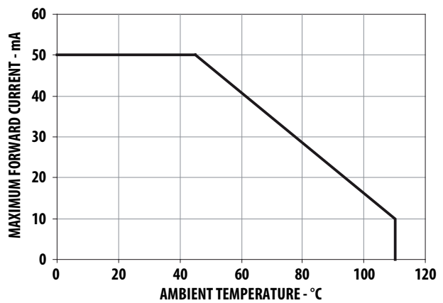
Figure 4a. Maximum Forward Current Vs. Ambient Temperature. Derated Based on T_{JMAX} = 125^{\circ}\text{C} , R\theta_{JA} = 300^{\circ}\text{C/W}
