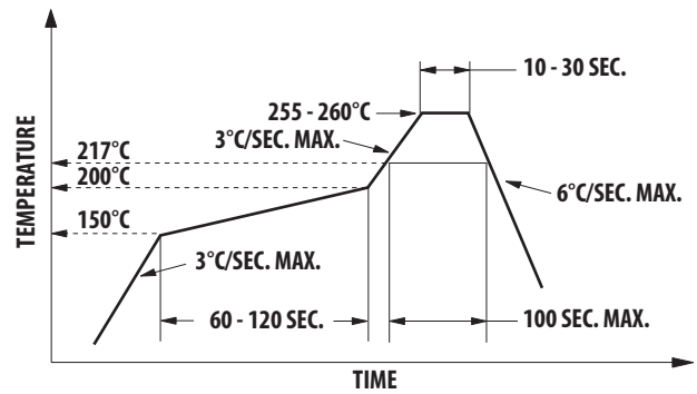
Figure 10b. Recommended Pb-Free Reflow Soldering Profile.
