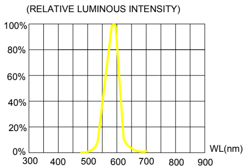
FIG.5 RELATIVE LUMINOUS INTENSITY VS.
